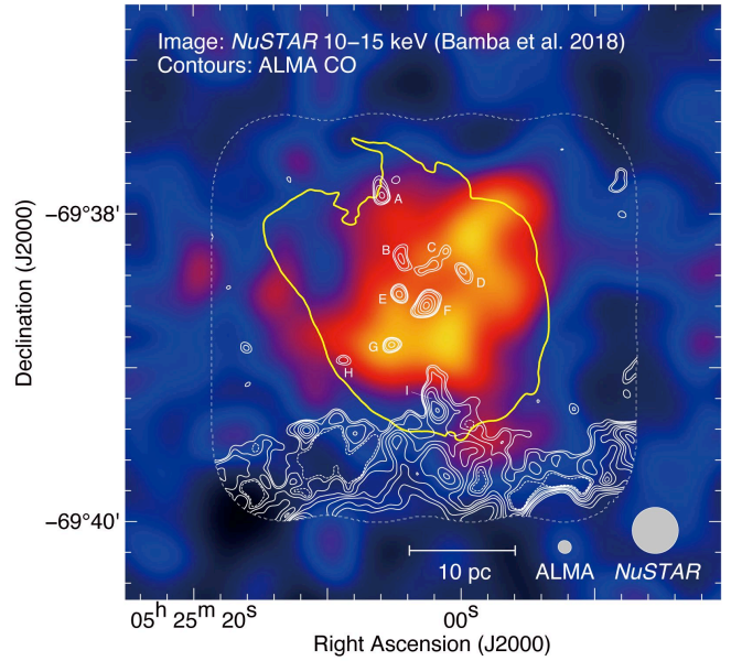
Figure 9. Map of hard X-ray emission ( E : 10–15 keV) obtained with NuSTAR (Bamba et al. 2018). The white and yellow contours indicate the ALMA ^{12}\text{CO}(J = 1-0) and the boundary of X-ray shell. The contour levels and integration velocity range of CO are the same as in Figure 5. The beam size and scale bar are also shown in bottom right corner for each panel. The CO clouds A–I are also indicated.
