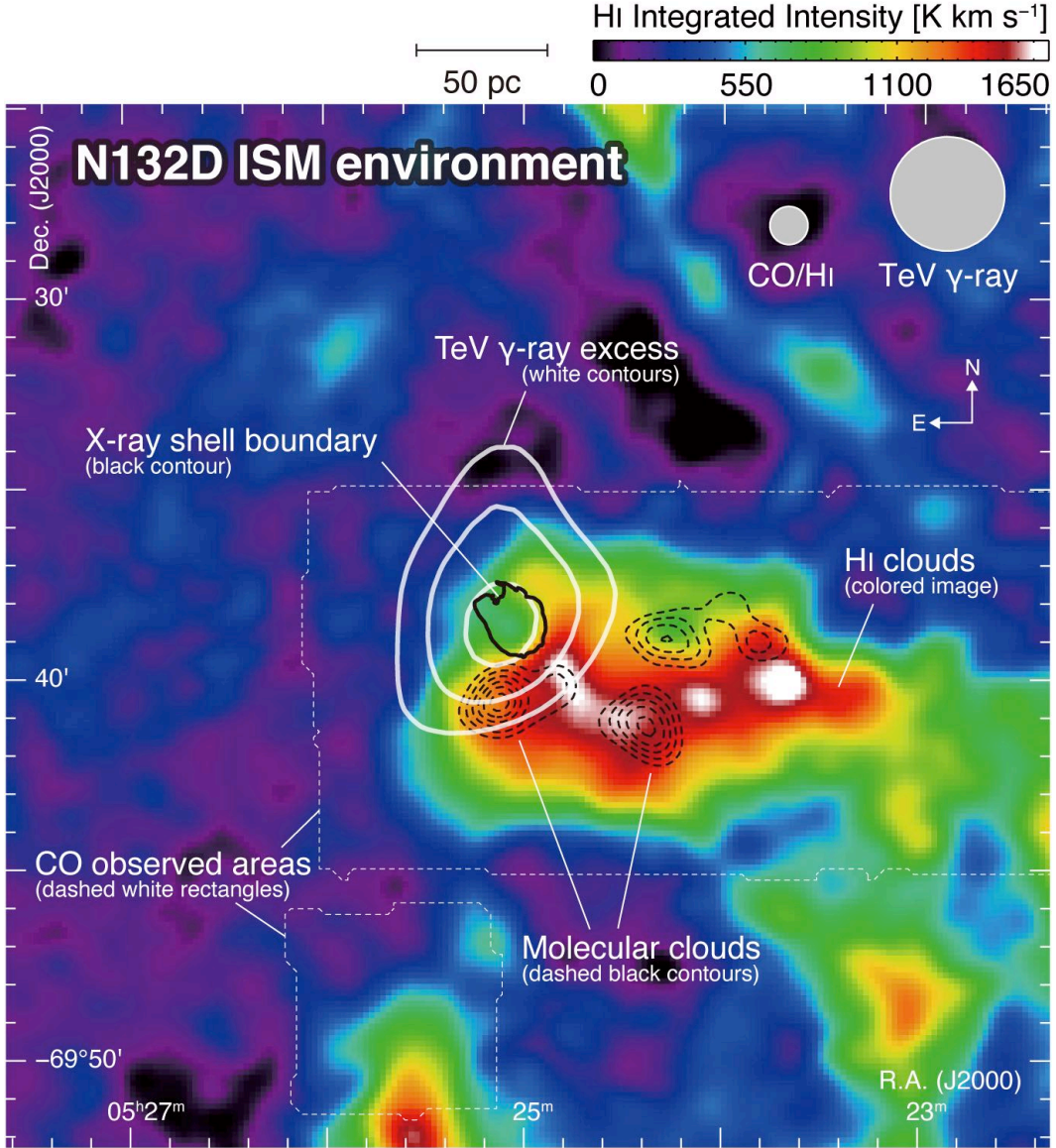
Figure 1. Integrated intensity map of the ATCA & Parkes HI (Kim et al. 2003, colored image ) overlaid with the Mopra ^{12}\text{CO}(J = 1-0) integrated intensity ( black dashed contours ), Chandra X-ray boundary of N132D (Borkowski et al. 2007, black solid contour ), and the H.E.S.S. TeV gamma-ray excess counts (H.E.S.S. Collaboration et al. 2015, white solid contours ). The CO data have been spatially smoothed to match the FWHM of HI ( \sim 60'' ). The integration velocity ranges of CO and HI are from 240 to 290 \text{km s}^{-1} , which cover 74 % of total integrated intensity of HI. The lowest contour level and intervals of CO are 6.3 \text{K km s}^{-1} ( \sim 9 \sigma ) and 2.1 \text{K km s}^{-1} ( \sim 3 \sigma ), respectively. The contour level of X-ray boundary is 0.3 \times 10^{-6} counts \text{pixel}^{-1} \text{s}^{-1} . The contour levels of TeV gamma-rays are 10, 14, and 18 excess counts. The dashed white rectangles indicate the observed areas of CO. The FWHM beam size of CO/HI and the PSF of TeV gamma-rays are also shown in top right corner.
