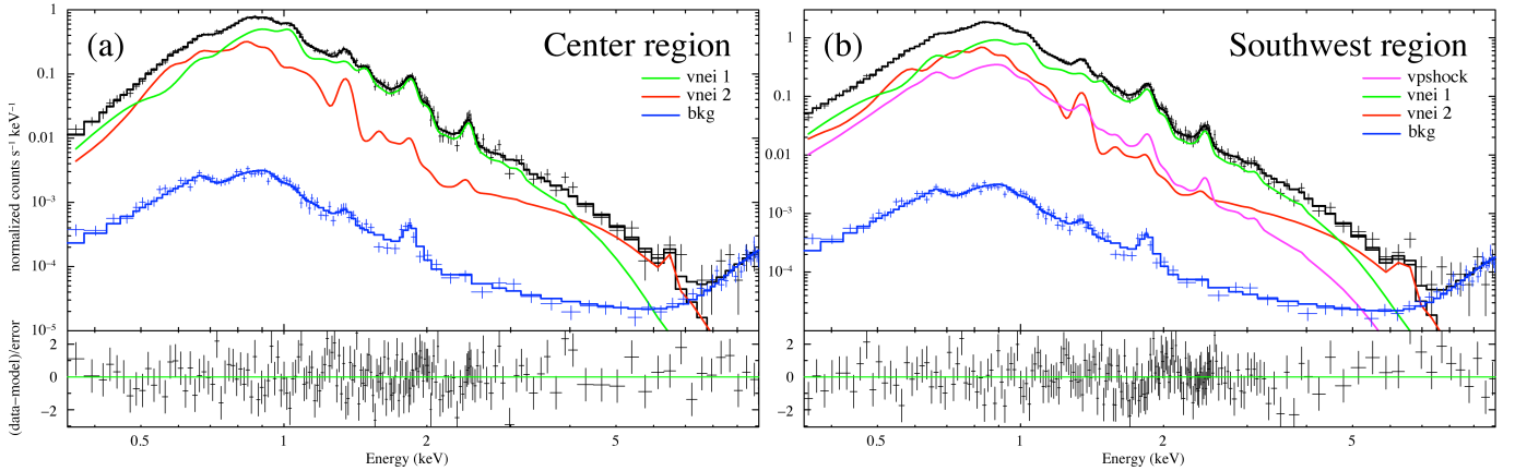
Figure 8. (a) ACIS-S spectra of the center (cloud F) and southwest (reference), with the best-fit models shown in the top panels. The magenta, green, red, and blue lines represent vshock , vnei 1, vnei 2, and background, respectively. The black lines represent the sum of the components. The bottom panels in each figure indicate (data - model) / error.
