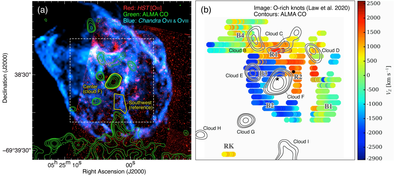
Figure 7. (a) RGB image of N132D obtained with the HST [O III] (red), ALMA 12 CO ( J = 1-0 ) (green contours), and Chandra O VIII emission produced using a novel method for source separation (blue, see Appendix). The integration velocity range and contour levels of CO are the same as in Figure 5. Regions enclosed by solid yellow lines are used for the X-ray spectral analysis (see Section 4.6). The dashed white box represents the area shown in Figure 7(b). (b) Radial velocity distributions of O-rich knots presented by Law et al. (2020). Superposed contours indicate the ALMA 12 CO ( J = 1-0 ), whose contour levels are the same as in Figure 5. The star and filled circle represent the center of O-rich knots and that of X-ray shell. Major knots — B1, B2, B3, B4, R1, R2, and RK (runaway knot) — from Morse et al. (1995) are also indicated.
