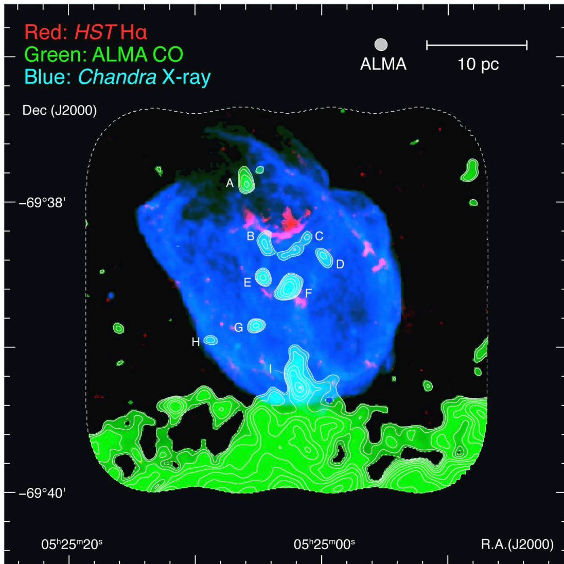
Figure 5. RGB image of N132D obtained with the HST H\alpha (red), ALMA ^{12}\text{CO}(J = 1-0) (green), and Chandra X-rays in the energy band of 0.5–7.0 keV (blue). The integration velocity range is from 262.0 \text{ km s}^{-1} to 268.4 \text{ km s}^{-1} . The contours represent the integrated intensity of CO, whose levels are 1.2 ( \sim 3\sigma ), 1.5, 2.0, 3.0, 4.0, 6.0, 9.0, 13.0, 18.0, and 24.0 \text{ K km s}^{-1} . The region enclosed by the dashed line indicates the observed area with ALMA. The CO clouds, named A–I, discussed in Section 4.3 are indicated.
