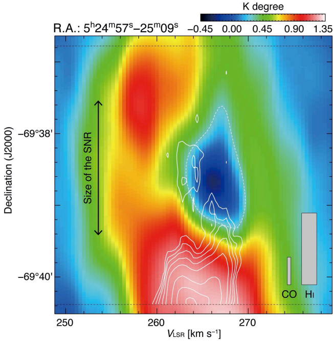
Figure 3. Position-velocity diagram of H I. Superposed white solid contours indicate ^{12}\text{CO}(J = 3-2) intensity. The integration range in Right Ascension is from 05^{\text{h}}24^{\text{m}}57^{\text{s}} to 05^{\text{h}}25^{\text{m}}09^{\text{s}} . The lowest contour and contour intervals of CO are 0.003 K degree and 0.005 K degree, respectively. The dashed white line delineates an H I cavity with the H I intensity of 0.3 K degree. The beam size and velocity resolution are also shown in bottom right corner. Horizontal dashed lines represent observed boundaries of CO.
