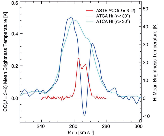
Figure 4. Averaged line profiles of ^{12}\text{CO}(J = 3-2) (red) and H I (blue and cyan) toward the SNR N132D. The blue and cyan spectra were extracted from regions of the inside and outside of the circle with a radius of 30'' at the center position of (\alpha_{\text{J2000}}, \delta_{\text{J2000}}) \sim (05^{\text{h}}25^{\text{m}}02^{\text{s}}.88, -69^{\circ}38'34''.8) . The red spectrum was produced by averaging the whole spectra shown in Figure 2b.
